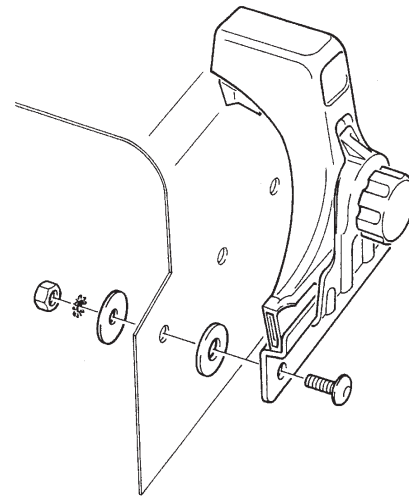
Montagevariante B Mounting alternative B
