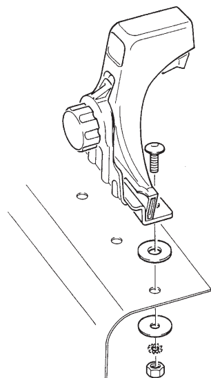
Montagevariante A Mounting alternative A
