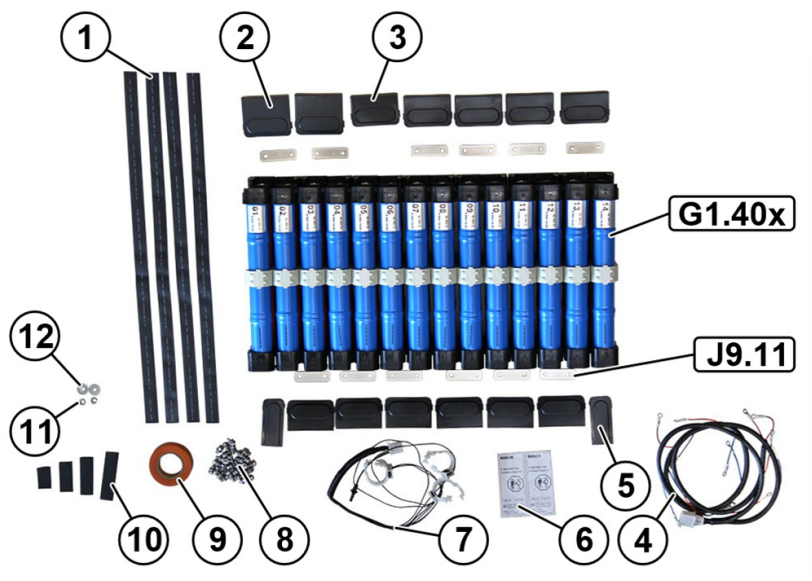
Figure 1 HV battery repair kit – scope of delivery
