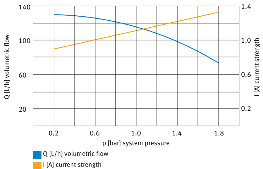
Fig. 2: Characteristic curves for current strength and volumetric flow in relation to system pressure (values may vary)
