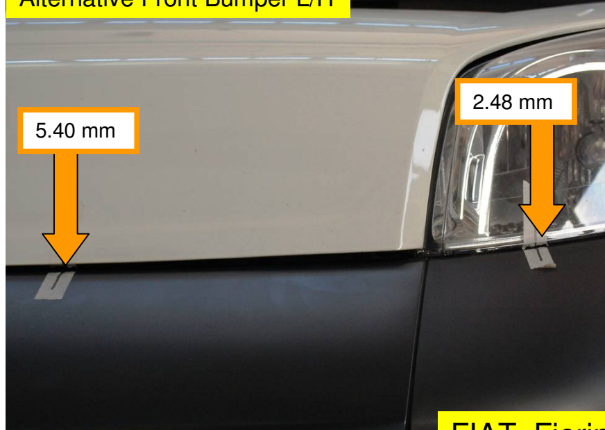
Alternative Front Bumper L/H
