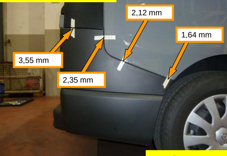
Original Rear Bumper R/H
